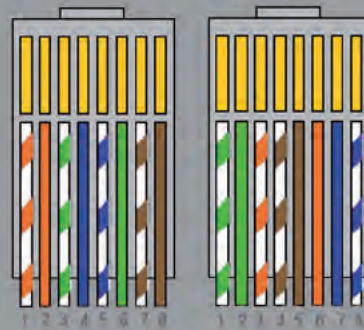
Cross-Connect Cable Termination 1 & 2 a.k.a Crossover Cable
